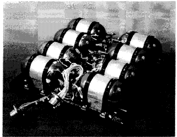
Figure-3: Mars Global Surveyor 2 Cell CPV Ni-H 2 Battery
