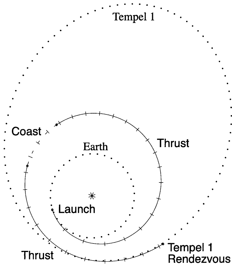
Figure 3 Earth – Tempel 1 Rendezvous
