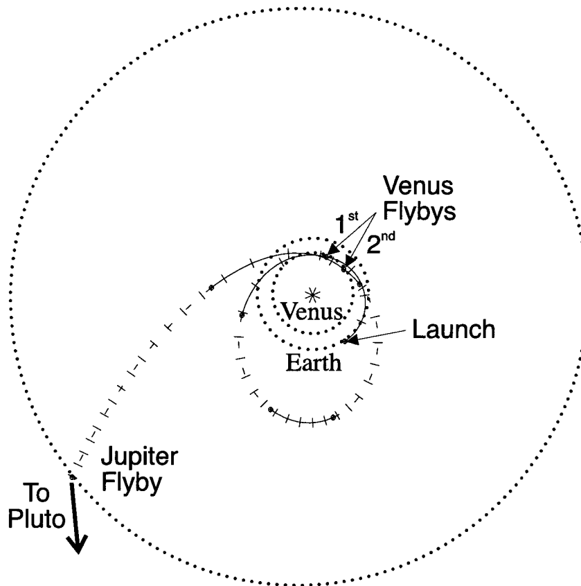
Figure 4 Earth – Venus – Venus – Jupiter Portion of Trajectory to Pluto
