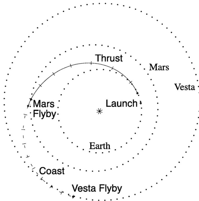
Figure 2 Earth – Mars – Vesta Flyby
