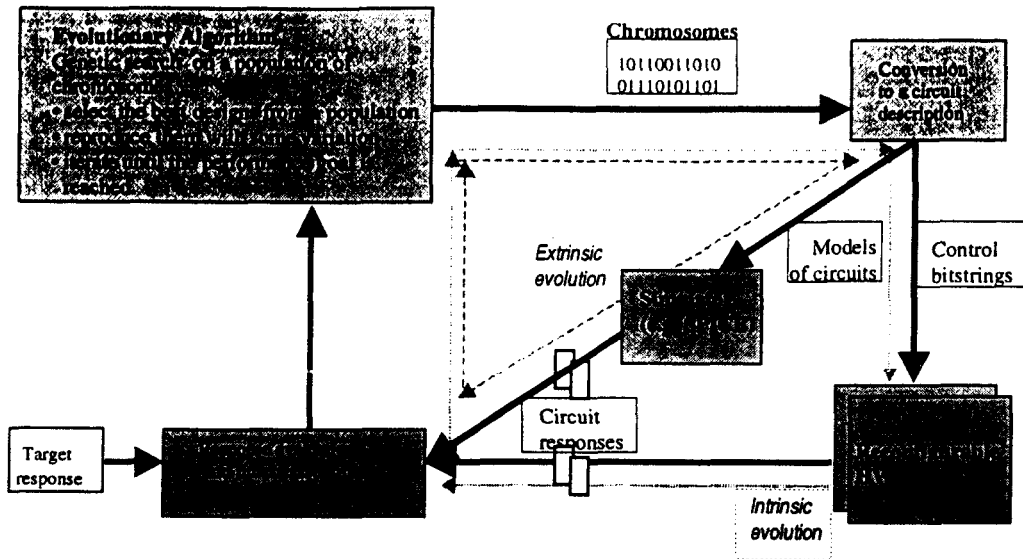
Figure 1: Evolutionary synthesis of electronic hardware
