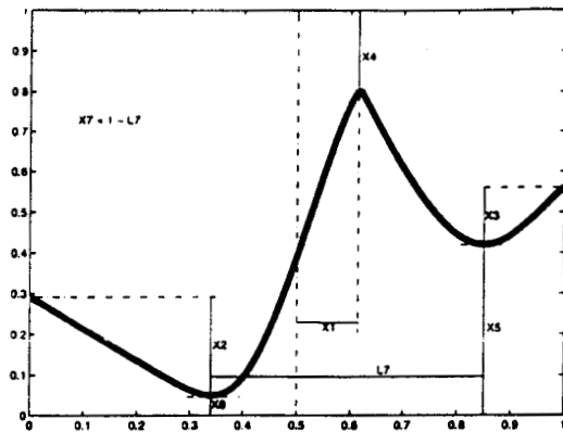
Figure 5: Parameters used for the specification of the fitness function. Fitness = f(x_1, \dots, x_7)
