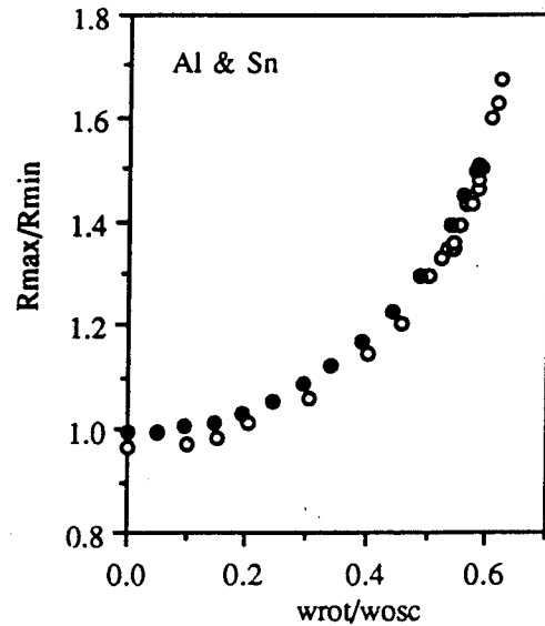
Fig. 5. Drop shapes of Al and Sn vs. rot. freq.
