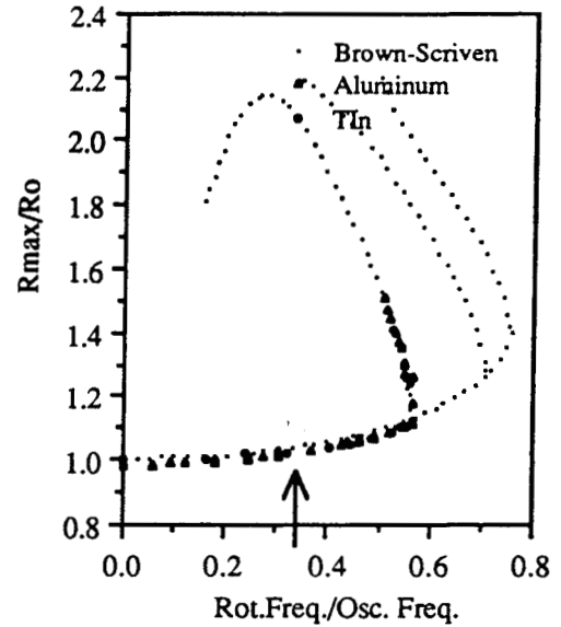
Fig. 3. Drop shape vs. rotation frequency.
