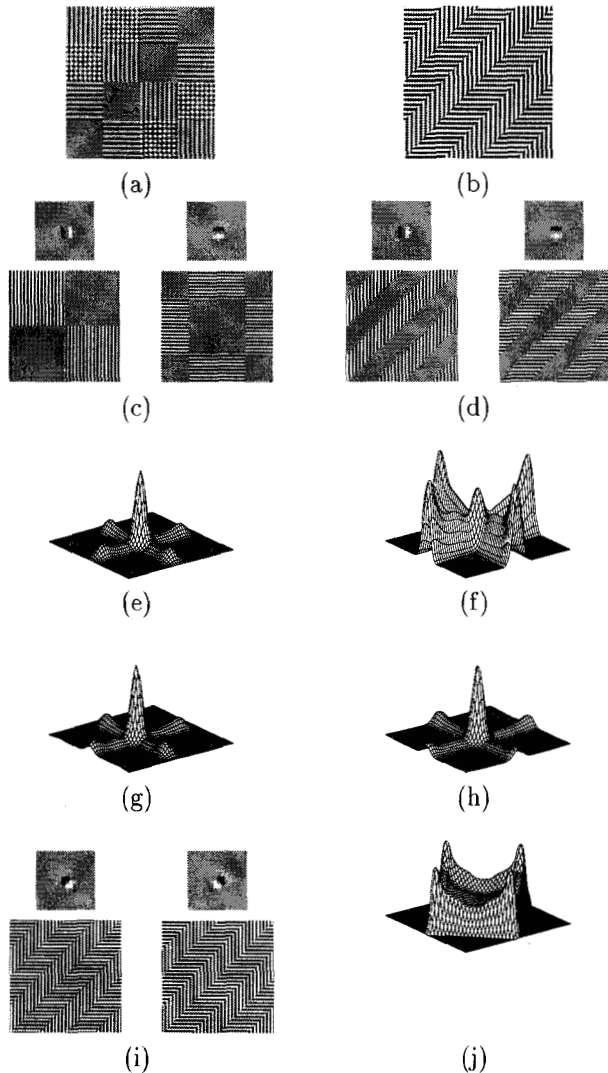
Figure 1: A case study (see text.) (a),(b): Textures A and B. (c),(d): The 0^\circ - 90^\circ kernels (upper row), and the filtered versions of the two textures (lower row.) (e),(f): The joint channel pdf's of the two textures. (g),(h): The separable approximations of the joint pdf's using the 0^\circ - 90^\circ filters. (i): The 45^\circ - 135^\circ kernels (upper row), and the filtered version of texture B (lower row.) (j) The separable approximation of the joint pdf of texture B using the 45^\circ - 135^\circ filters.
