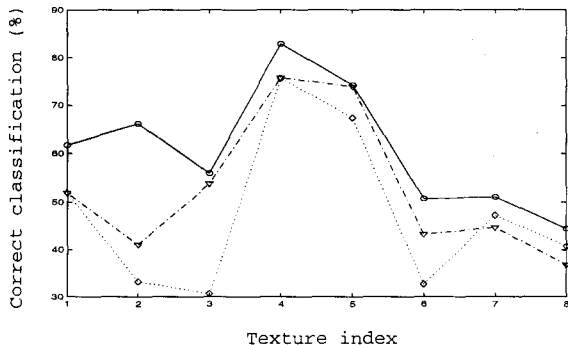
Figure 2: Supervised classification test (see text). The system is trained and tested on the eight textures shown above. The plots represent the percentage of correct classification for each texture. Solid line: using ICA transformation. Dot-dashed line: using PCA transformation. Dotted line: without transformation.
