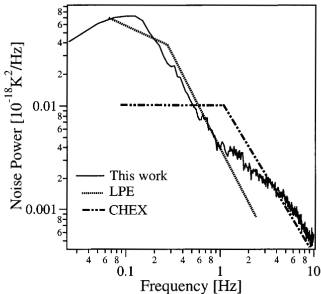
Figure 4. Noise power spectral density of the thermometer at T = 2.17\text{K} .
