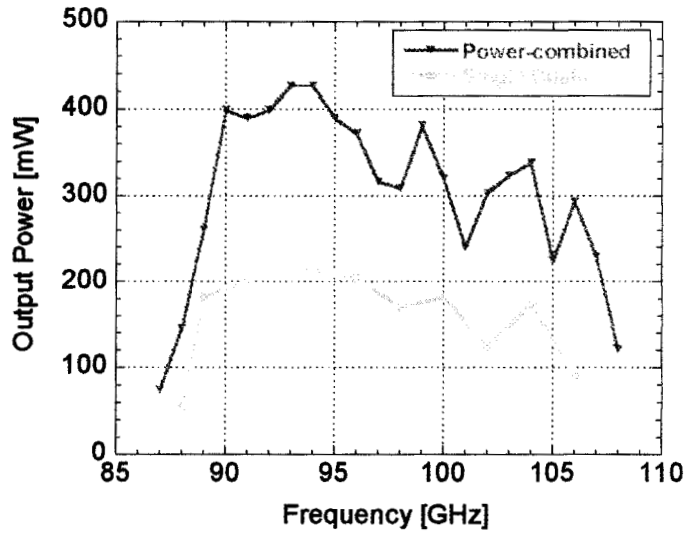
Figure 10. Left, schematic showing configuration of amplifiers and magic tees. DA=microstrip driver amplifier; PA = microstrip power amplifier. At right, output power as a function of frequency is shown for a single amplifier chain and the magic-tee power-combined chain, measured at room temperature.
