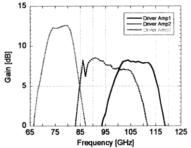
Figure 3 a. (Left) Chip photograph of microstrip driver amplifier covering 71-82 GHz. 3b. (Right) Small-signal gain of the three microstrip driver amplifiers. Driver Amp3 is the result of the chip in the photograph in 3a.
