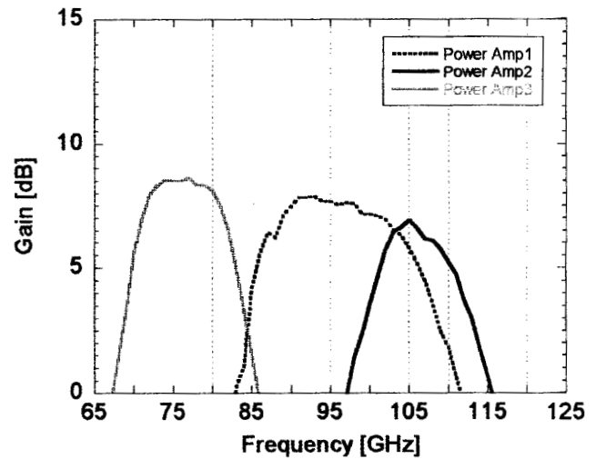
Figure 4 a (Left). Chip photograph of microstrip power amplifier covering 89-105 GHz. 4b(Right) Small-signal gain of the three microstrip power amplifiers. The Power Amp 1 curve is the result of the chip in the photograph of 4a.
