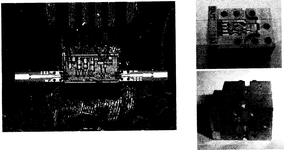
Figure 5. Left-hand photograph shows CPW driver chip with waveguide-to-microstrip probe transitions in a waveguide mount. Upper right photo shows the overview of the waveguide mount without its cover. Lower right photo shows the waveguide module with cover intact.
