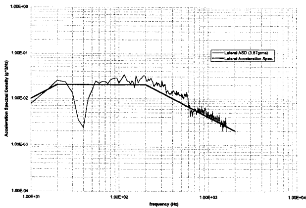
Figure 11. DS1 Spacecraft Full Level Input Acceleration Spectral Density for Lateral Vibration Test
