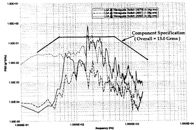
Figure 12. Acceleration Inputs to LGA Interface in DS1 Spacecraft Vertical Random Vibration Test
