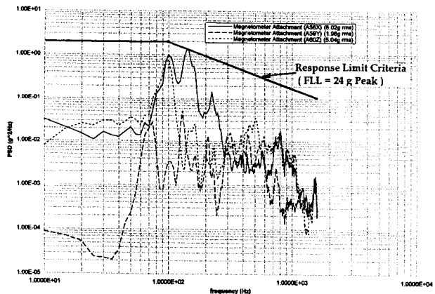
Figure 10. Magnetometer Attachment Response Spectral Density in DS1 Spacecraft Vertical Random Vibration Test
