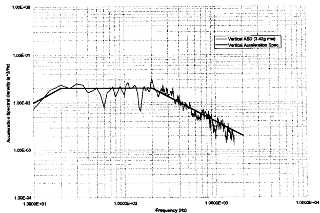
Figure 8. Full Level Input Acceleration Spectral Density in DS1 Spacecraft Vertical Random Vibration Test
