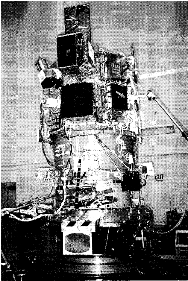
Figure 2. DS1 Spacecraft on Shaker for Vertical Vibration Testing
