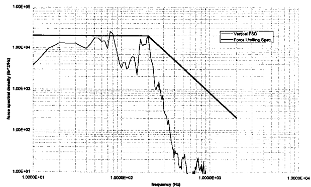
Figure 9. Total Vertical Force Measured in DS1 Spacecraft Vertical Random Vibration Test
