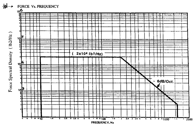
Figure 5. DS1 Spacecraft Random Vibration Force Limit Specification
