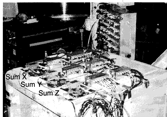
Figure 7. Summing of 24 Force Measurements in X, Y, & Z Directions
