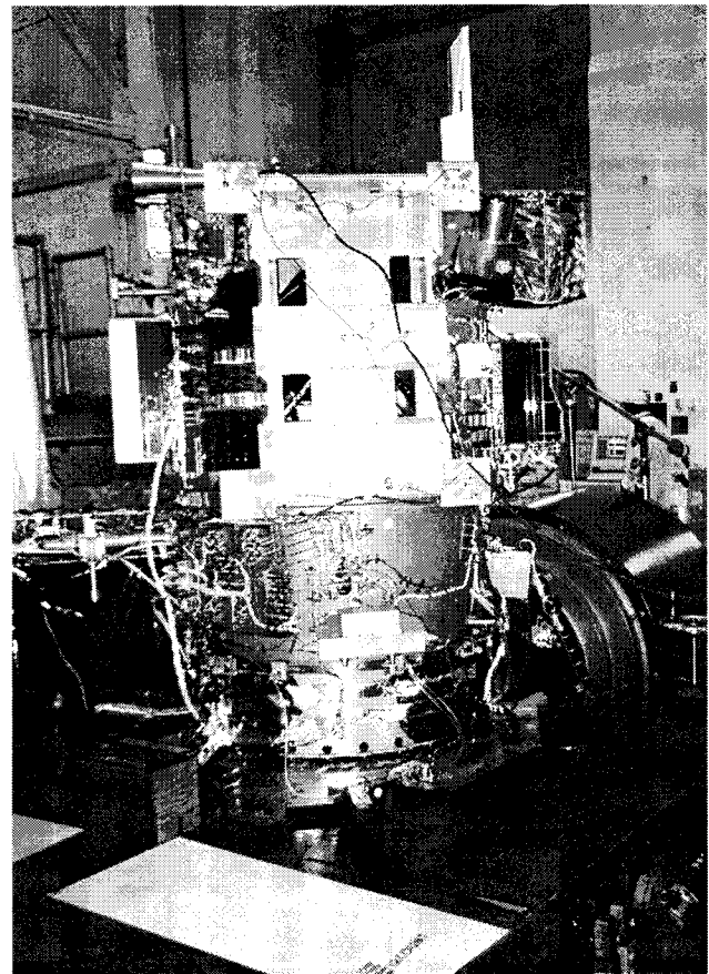
Figure 3. DS1 Spacecraft on Shaker for Lateral Vibration Testing
