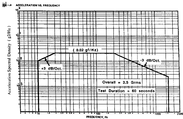
Figure 4. DS1 Spacecraft Random Vibration Acceleration Specification
