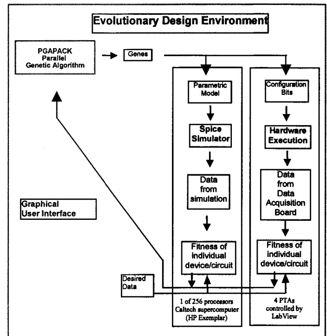
Figure 3 Environment for evolutionary design.
