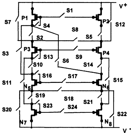
Figure 1 Module of the Programmable Transistor Array
