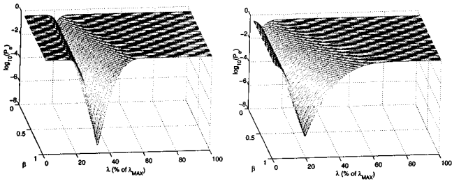
Fig. 6. \log_{10}(P_e) as defined in Eq. (12) plotted as a function of the threshold \lambda and the multiplicative attenuation \beta for both day (left) and night (right) conditions, for the case of worst case a priori probabilities. The deep valley in the plot traces the path of the optimal threshold for different \beta . It can be seen that for lower values of \beta the optimal threshold is lower, while higher values of \beta require higher thresholds.
