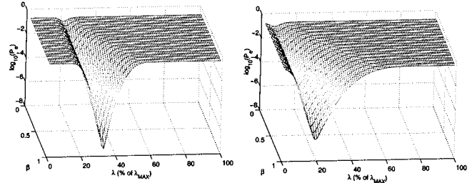
Fig. 7. \log_{10}(P_e) as defined in Eq. (12) plotted as a function of the threshold \lambda and the multiplicative attenuation \beta for both day (left) and night (right) conditions, for the case of equal a priori probabilities. See also Fig. 6.
