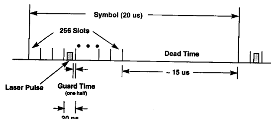
Fig. 1. Pulse Position Modulation timing diagram: the slot width T_s is 20 ns; the symbol width T_s is 20 \mu s; there are N_s = 256 slots in a symbol, within which a signal pulse can occur; there are N_d \approx 750 dead-time slots in a symbol; and there are about one thousand ( N_s + N_d ) total slots per symbol.
