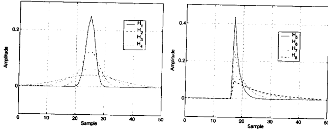
Fig. 2. Illustration of Gaussian (left), and exponential (right) pulse shapes used in the simulations. The sampling rate is 800 MHz (16 samples per 20 ns slot). For the Gaussian pulses, three PPM slots (48 samples) are illustrated with the signal slot in the center. The exponential pulses begin at the start of the signal slot in order to maximize photon collection within the signal slot.
