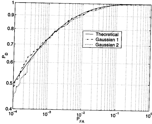
Fig. 5. Illustrated here are a “theoretical” ROC curve for \beta = 0.2900 ; and two experimentally obtained ROC curves: “Gaussian 1” for the case where \sigma = 0.2T_s and \alpha = 0.30 , corresponding to \beta = 0.2963 , and “Gaussian 2” for the case where \sigma = 0.6T_s and \alpha = 0.50 , corresponding to \beta = 0.2977 .
