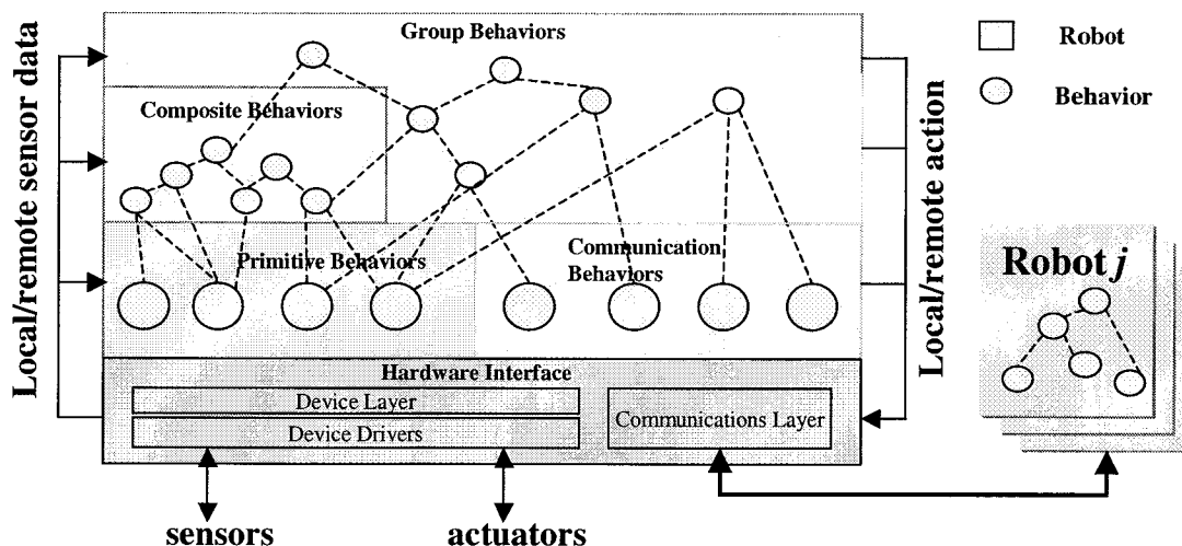
Figure 1 Schematic overview of CAMPOUT and its hierarchical organization in terms of primitive behaviors, composite behaviors built from primitive behaviors and group behaviors that are composed from coordination of behaviors across multiple robots. Each robot runs an instance of this architecture and coordinates activities through group behaviors, which is facilitated through the communications behaviors.
