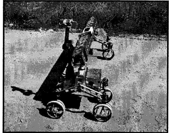
Figure 3 Transport of an extended object requiring the tightly coupled co-ordination of multiple robot. (left) Column formation for long traverse. (right) Row formation for precision placement.
