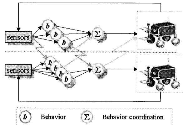
Figure 2 Networked robotics and resource sharing elements of CAMPOUT that enable definition of group coordination behaviors.
