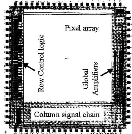
Figure 2. Imager layout with component blocks.
