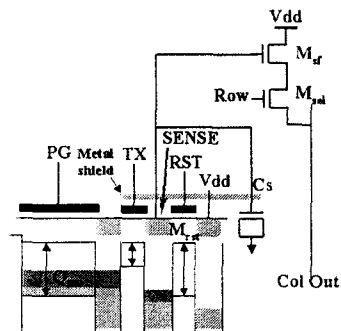
Figure 1. Schematic diagram of the frame-difference imager pixel circuit. The sense node, covered by metal for optical shielding, provides in-pixel frame memory. The FET capacitor ( C_s ) enables high-flux operation.
