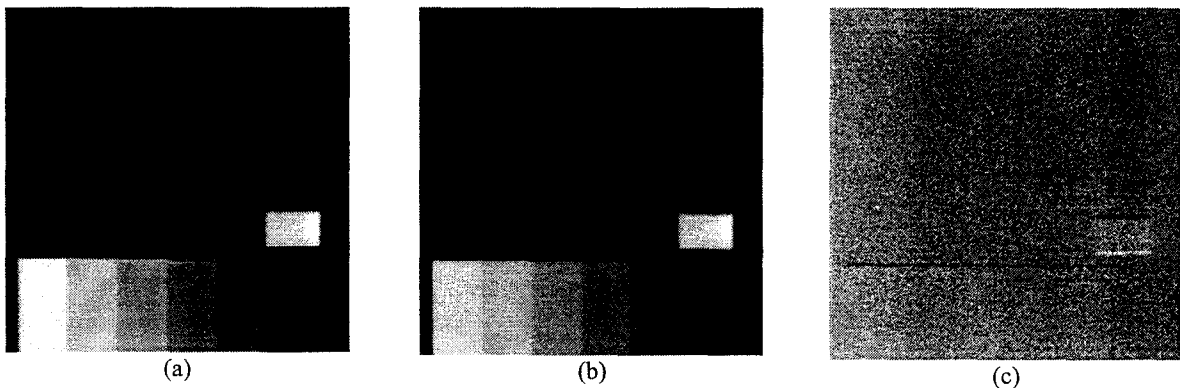
Figure 3. (a) Direct mode image of gray scale bar-pattern with >180\times reflectivity variation, under "white light" illumination. (b) Difference mode image without error correction. (c) Difference mode image after error correction.
