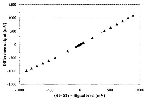
Figure 5. Frame-difference output as a function of the actual intensities in the two frames under flat-field, red LED illumination.
