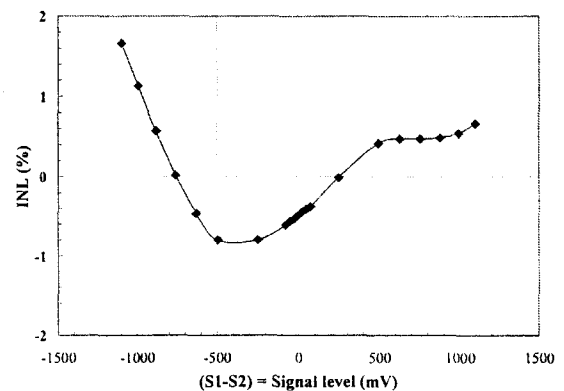
Figure 6. Integral Non-Linearity (INL) of the difference output after leakage correction, under flat-field, red LED illumination.
