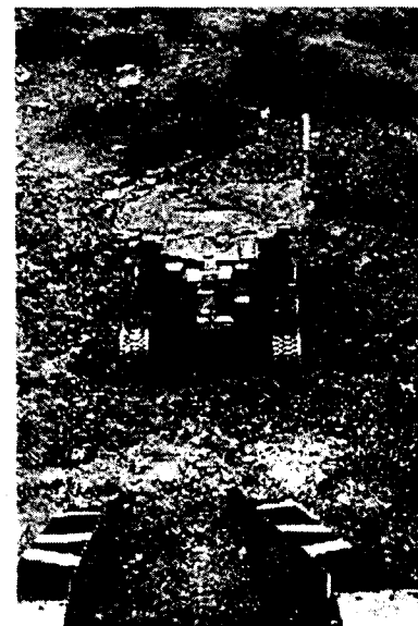
Figure 8: (Left) Operational scenario for rover rendezvous with Mars lander/ascent vehicle (the pictures within show our Sample Return Rover research prototype; (Right) as implemented on FIDO, final approach in progress
