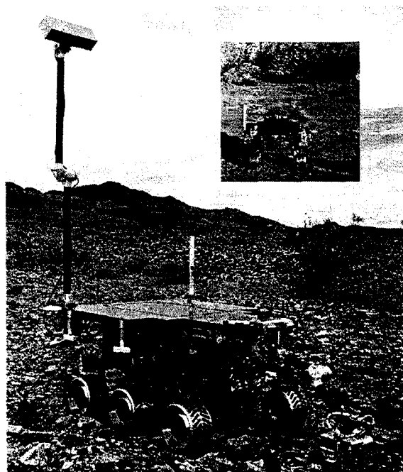
Figure 1: FIDO Rover during its 1999 field testing activities on a cobbled bed, Silver Lake, California, with mast/instrument arms extended. Inset depicts the continuous traverse of a nearby sand wash, rover seen in rear view, mast/instrument arms now stowed.
