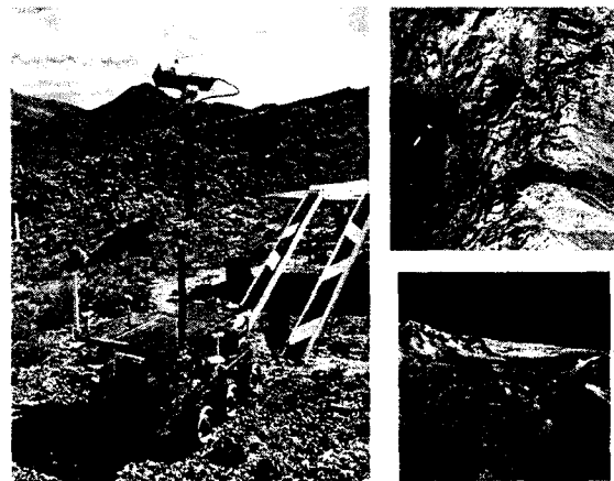
Figure 3: FIDO Rover at the Nevada blind field test, egress from lander complete, and beginning its science mission. Pictures at upper and lower right: composite LANDSAT data and LANDSAT overlay of 3D TIMS reconstruction. See also http://wufs.wustl.edu/fido
