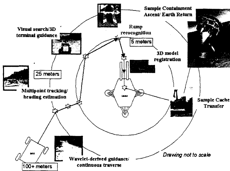
Figure 8: (Left) Operational scenario for rover rendezvous with Mars lander/ascent vehicle (the pictures within show our Sample Return Rover research prototype; (Right) as implemented on FIDO, final approach in progress
