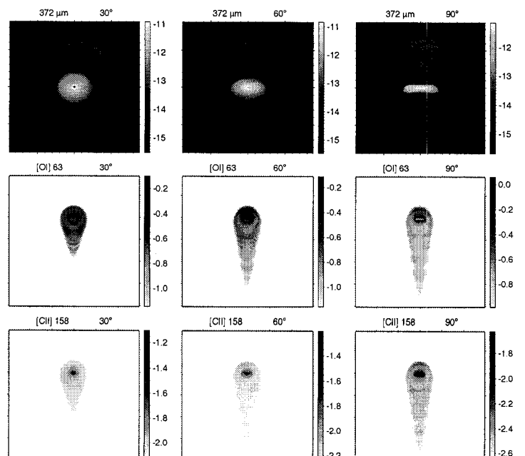
Fig. 6: Line and Continuum maps for the low-mass system shown in Fig. 2 for wavelengths and viewing angles as indicated. The scale of the 3 top frames is 1800x1800 AU and of the bottom 6 frames is 6000x6000 AU.
