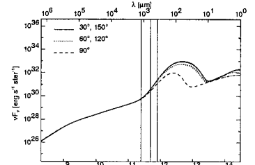
Fig. 4: SED of the low-mass system shown in Fig. 2.
