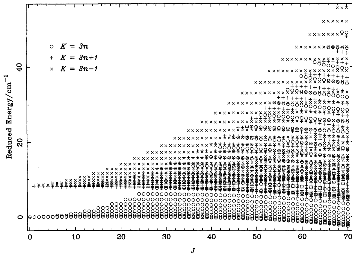
Reduced Energy = E - (B+C)J(J+1)/2 vs J
