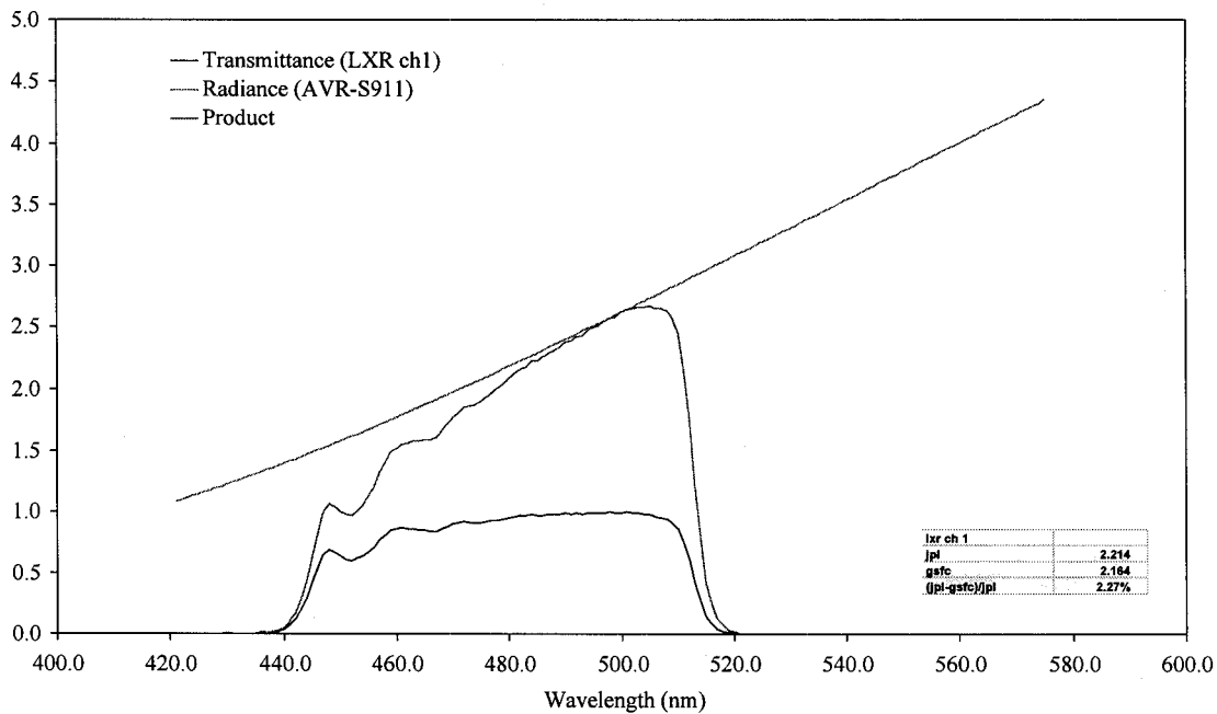
Figure 5. Comparison of the AVIRIS radiometric standard to the Landsat Transfer Radiometer Channel 1.
