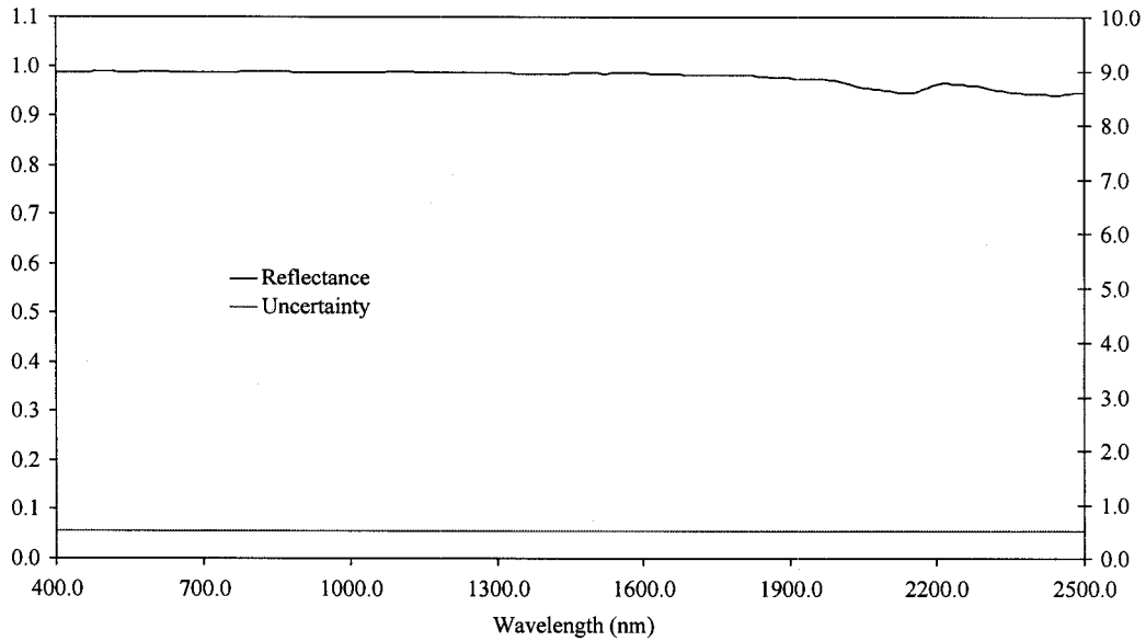
Figure 3. Panel reflectance as a function of wavelength, corrected to \{0^\circ, 45^\circ\} BRDF.
