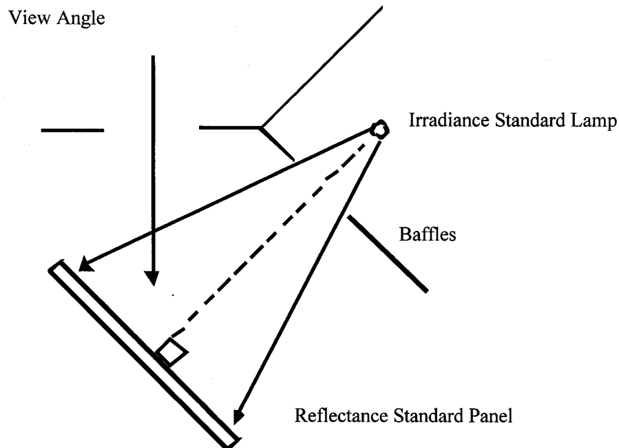
Figure 1. AVIRIS Portable Radiance Fixture Schematic Diagram
