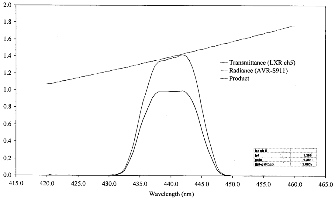
Figure 9. Comparison of the AVIRIS radiometric standard to the Landsat Transfer Radiometer Channel 5.
