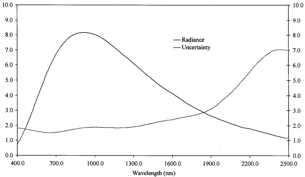
Figure 4. Spectral radiance from AVIRIS portable radiance standard with estimated uncertainty.
