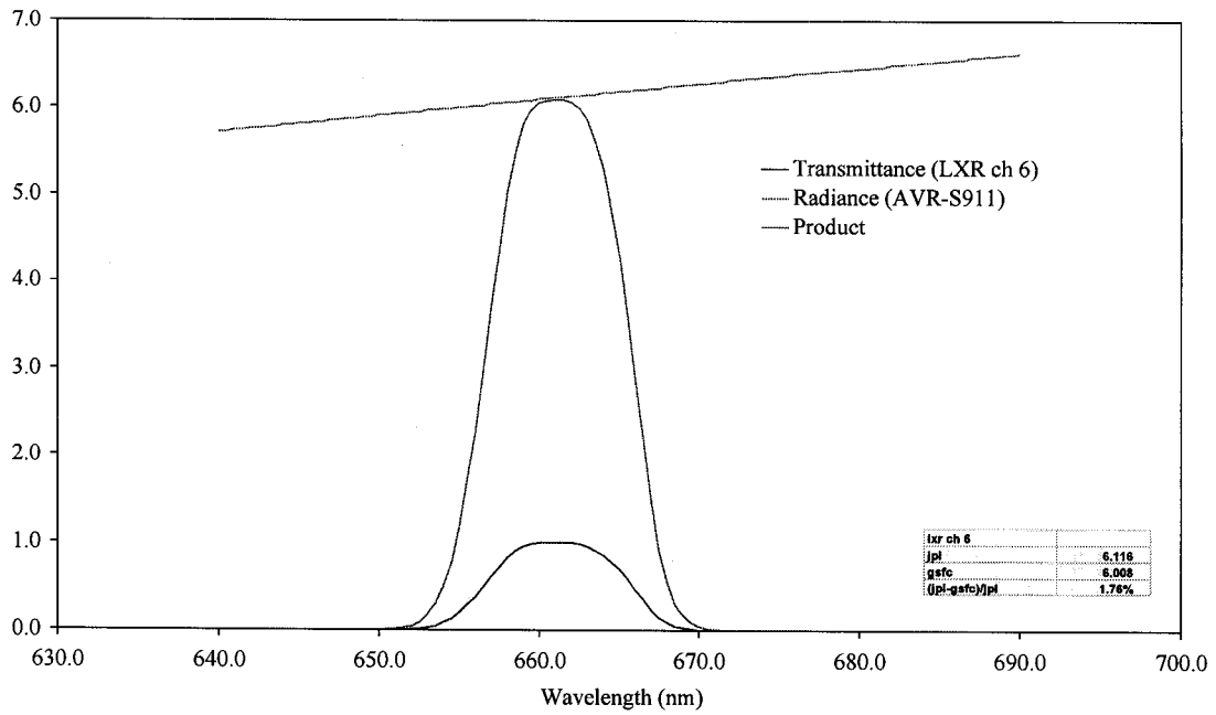
Figure 10. Comparison of the AVIRIS radiometric standard to the Landsat Transfer Radiometer Channel 6.
