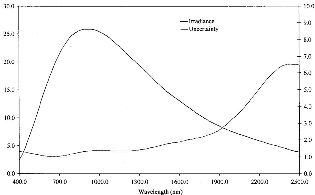
Figure 2 Spectrum of irradiance lamp source with uncertainty.
