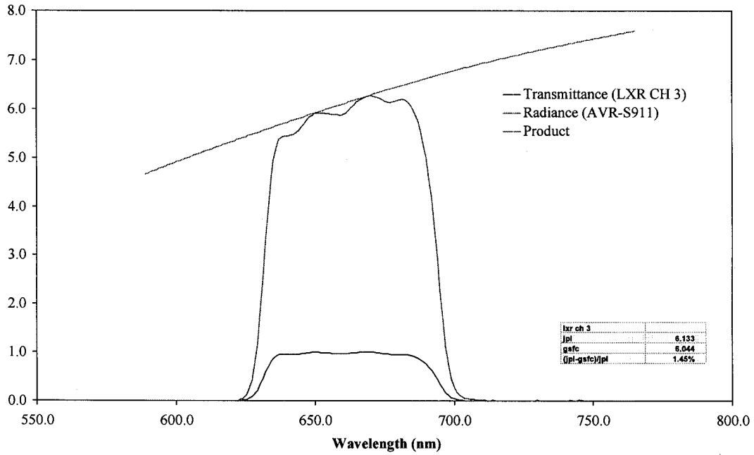
Figure 7. Comparison of the AVIRIS radiometric standard to the Landsat Transfer Radiometer Channel 3.
