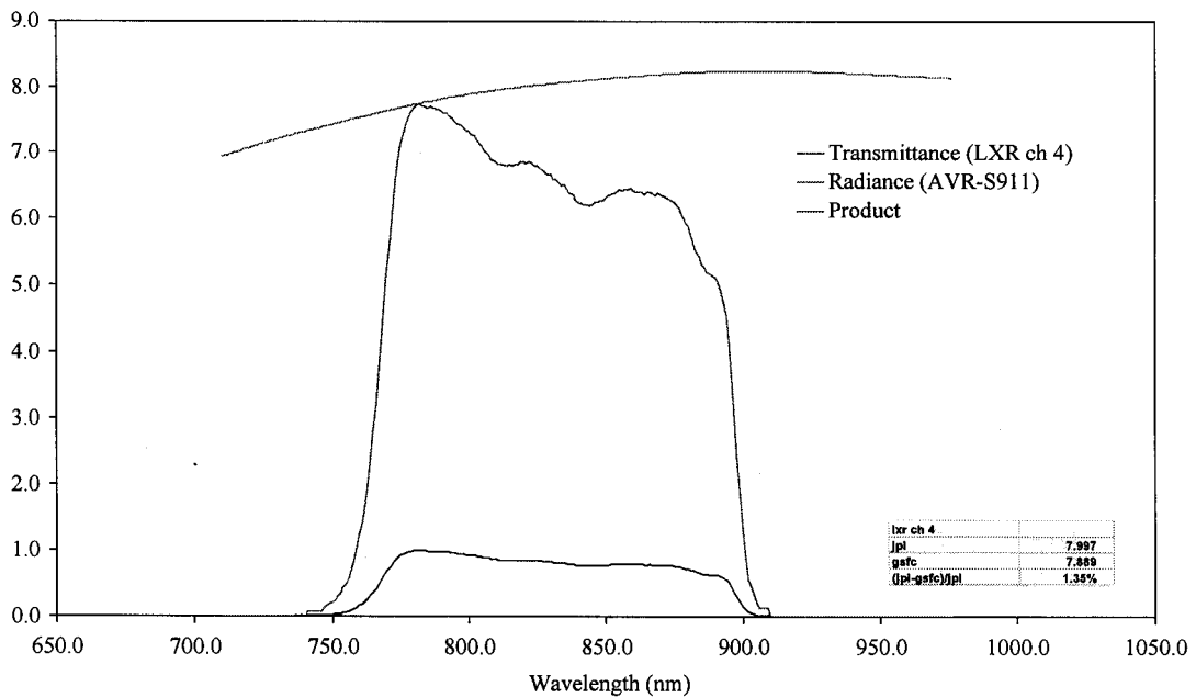
Figure 8. Comparison of the AVIRIS radiometric standard to the Landsat Transfer Radiometer Channel 5.
